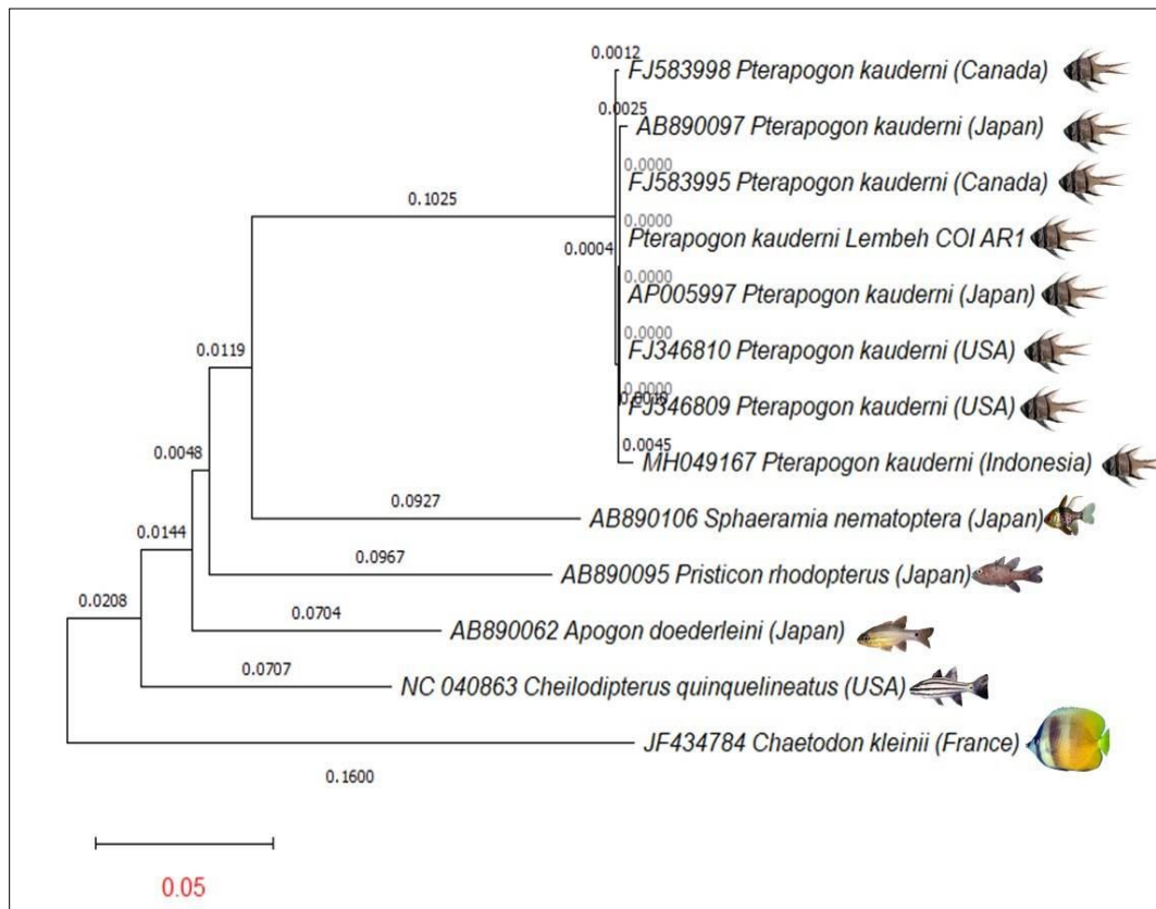
Figure 3. The phylogenetic tree of Pterapogon kauderni .
